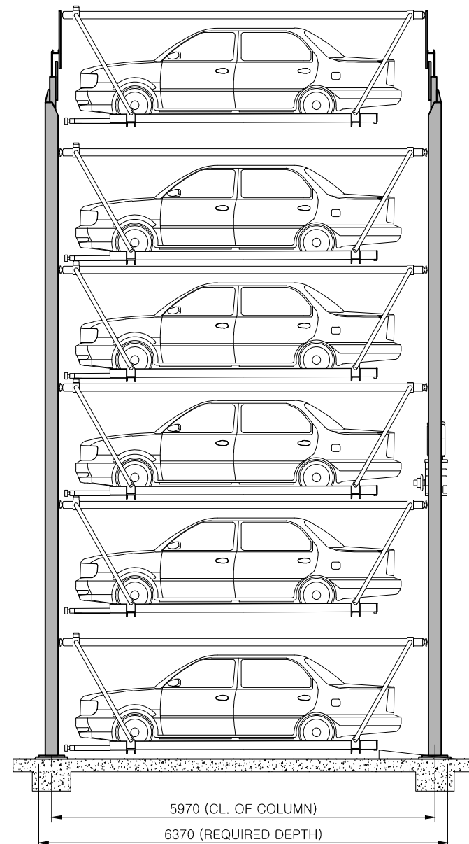
SIDE ELEVATION
