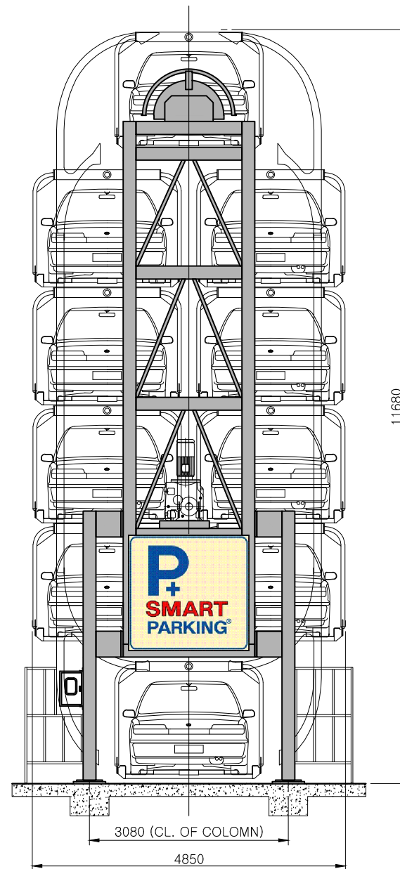
FRONT VIEW
