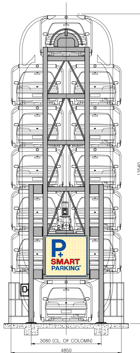
FRONT VIEW
