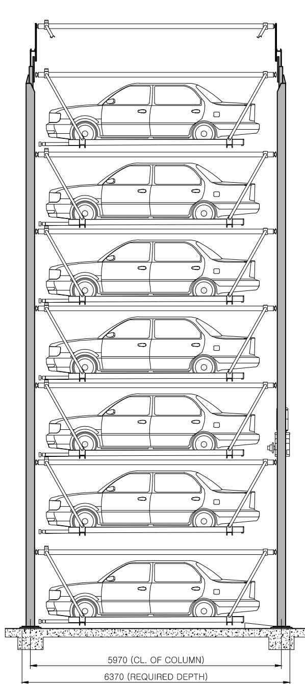
SIDE ELEVATION
