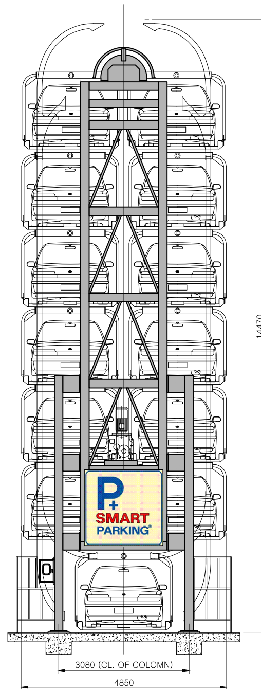
FRONT VIEW
