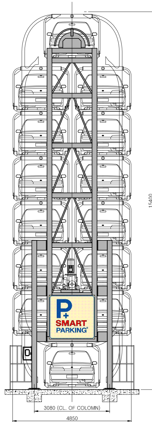
FRONT VIEW
