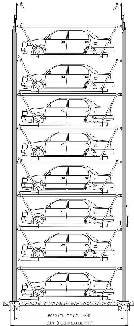
SIDE ELEVATION
