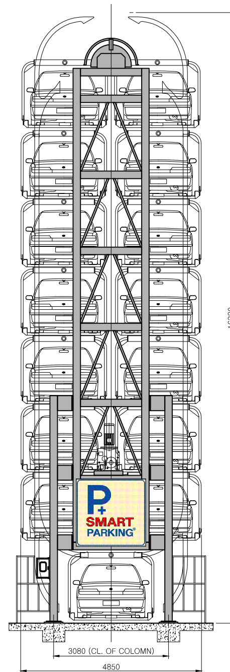
FRONT VIEW
