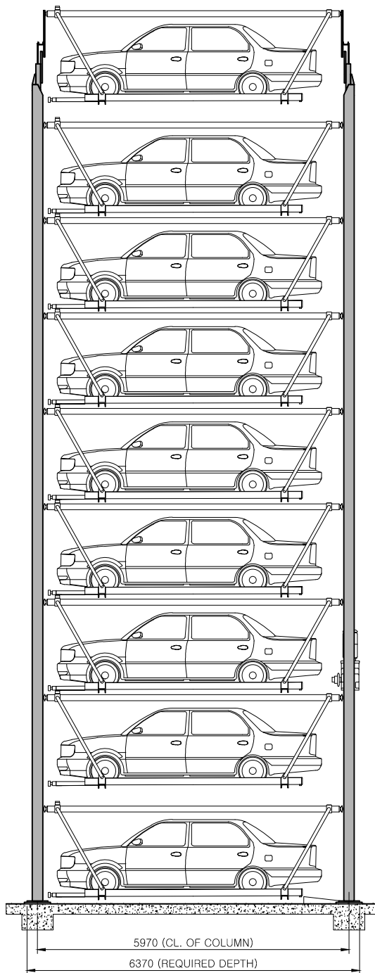
SIDE ELEVATION
