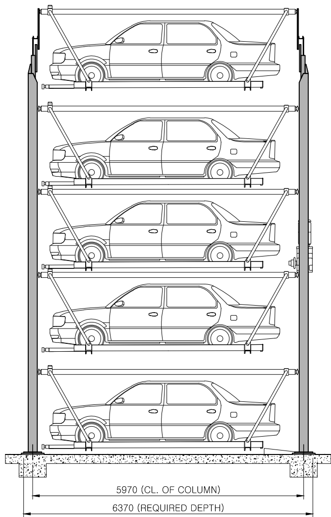
SIDE ELEVATION
