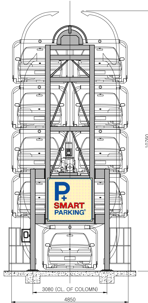
FRONT VIEW
