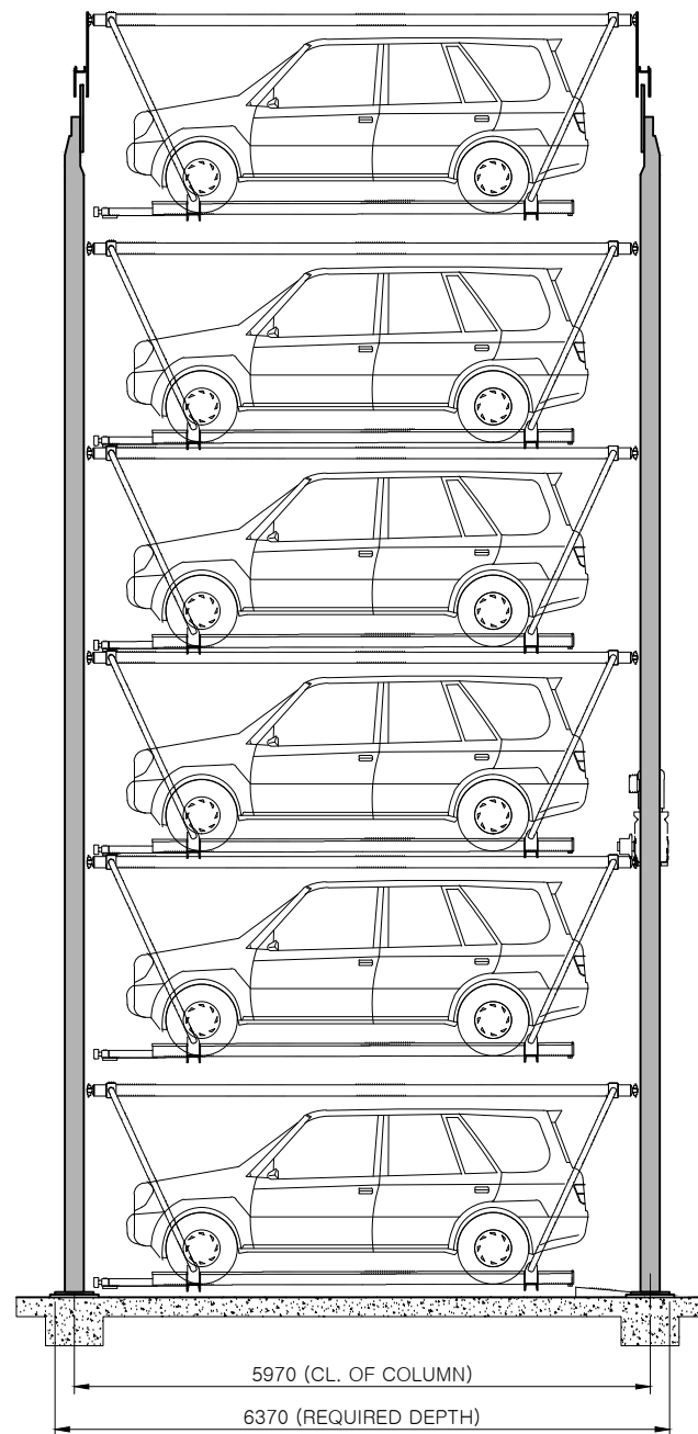
SIDE ELEVATION
