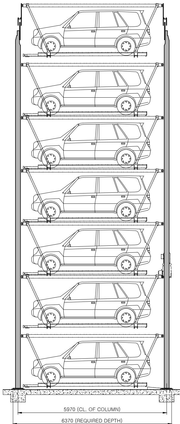
SIDE ELEVATION
