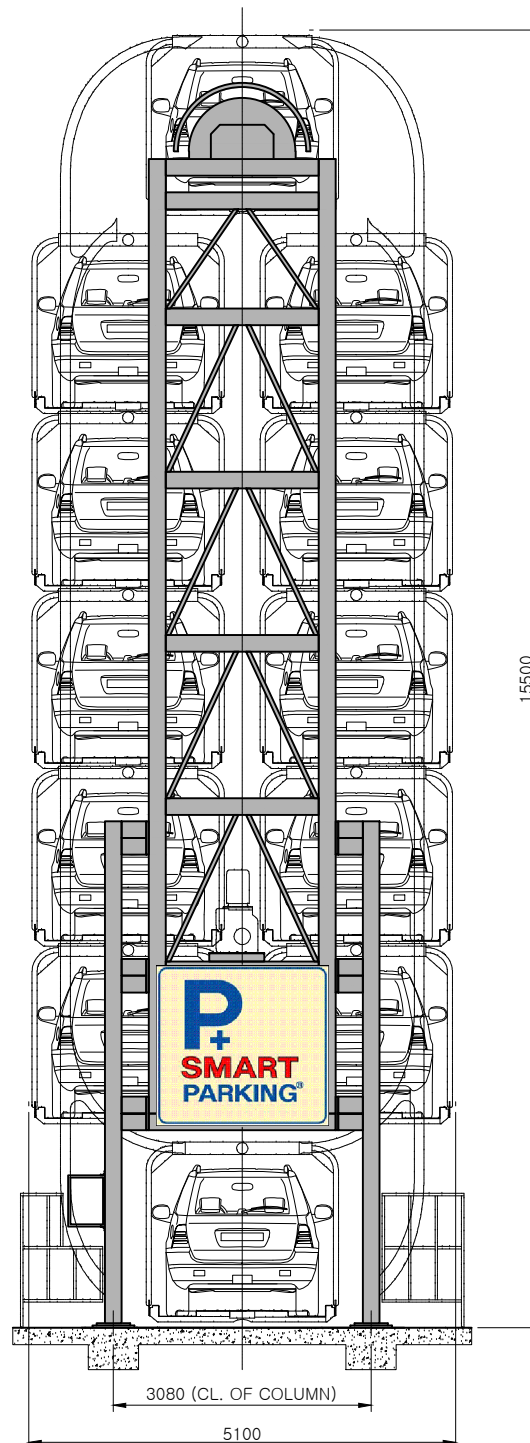
FRONT VIEW
