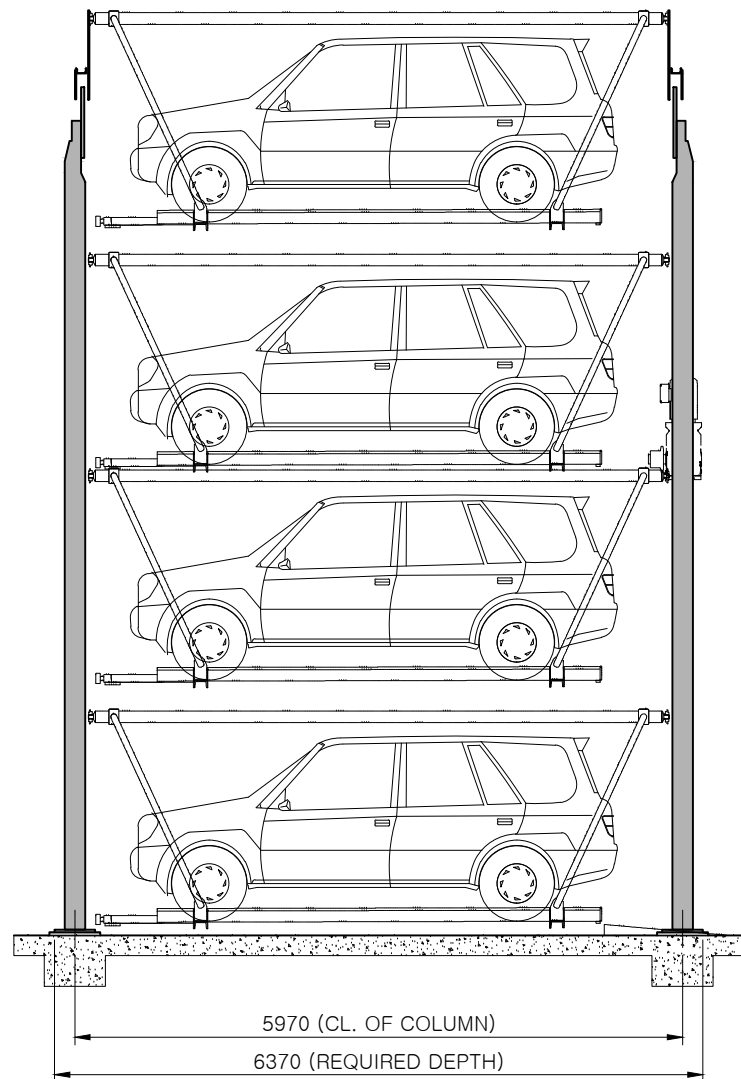
SIDE ELEVATION
