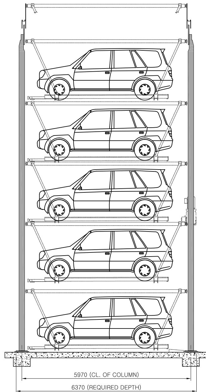
SIDE ELEVATION
