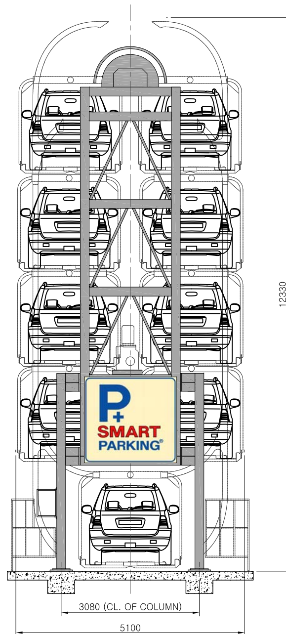
FRONT VIEW
